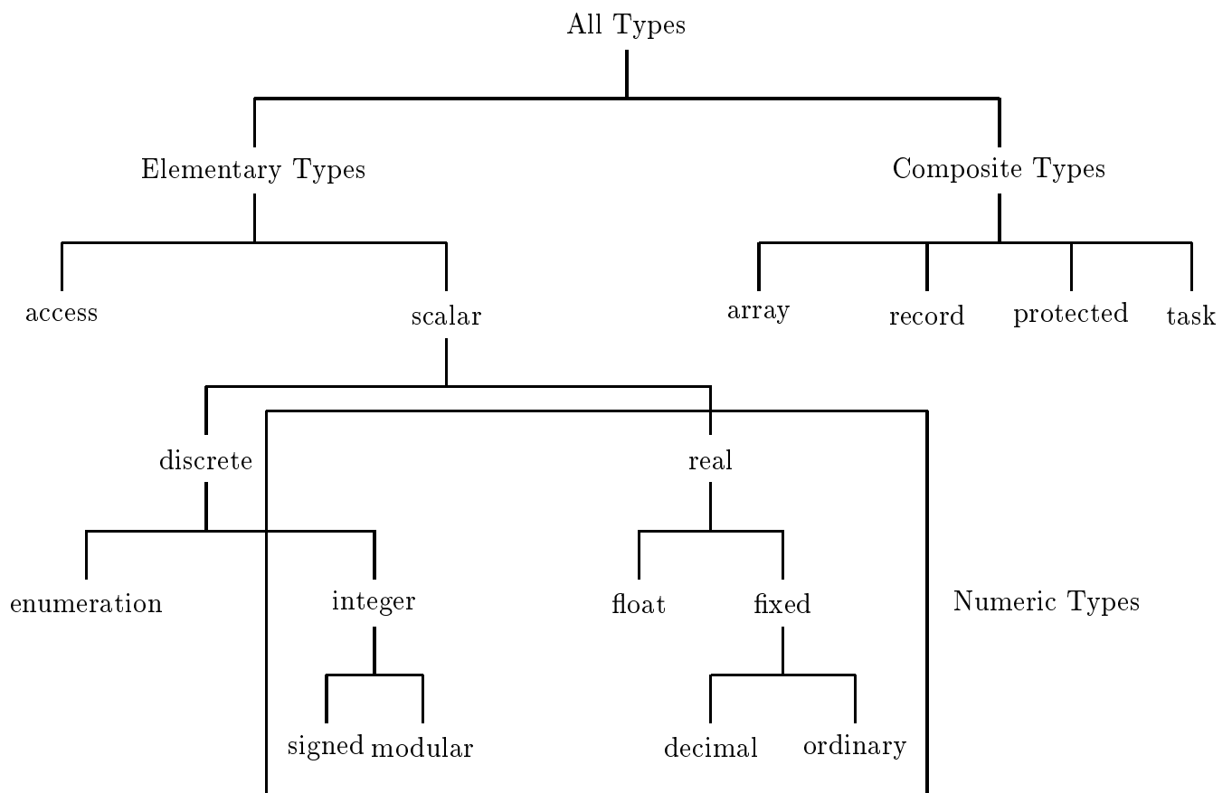
Ada-95 Type Hierarchy.
