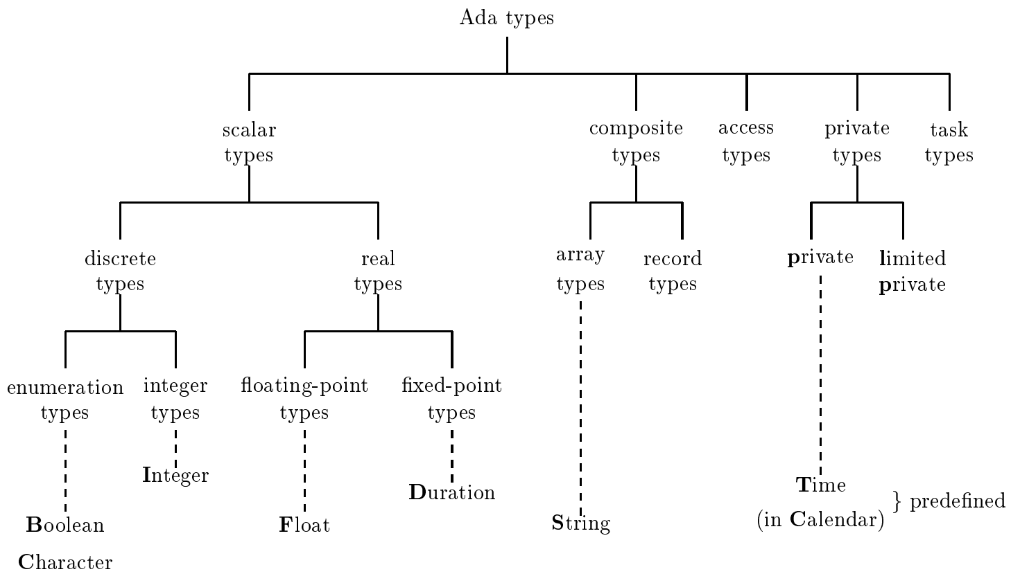
Classification of data types in Ada-83.
